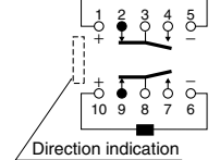
2-coil latching
